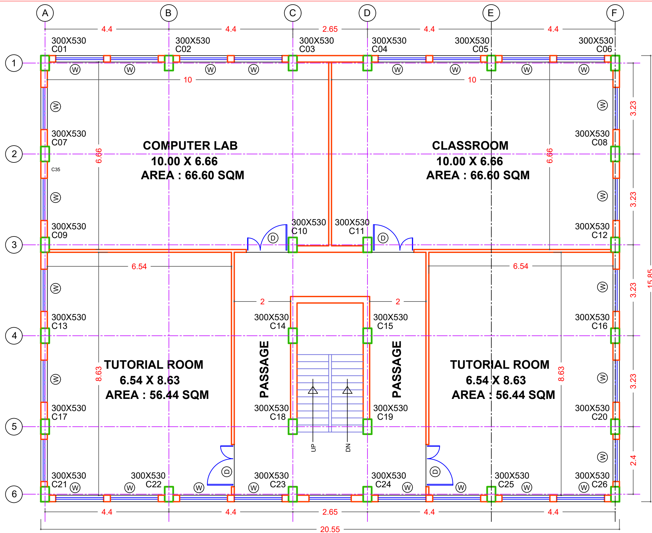
SECOND FLOOR ( MULTI-PURPOSE HALL BUILDING )
